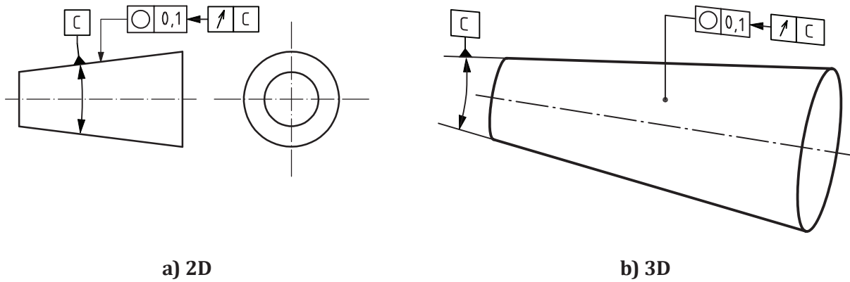
Figure 100 — Roundness indication
