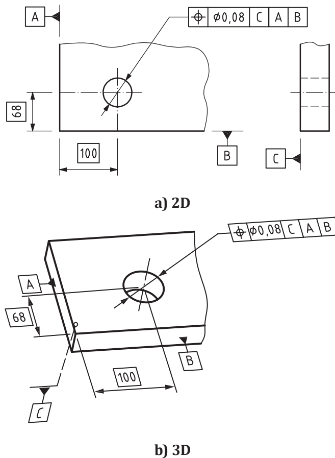
Figure 154 — Position indication
