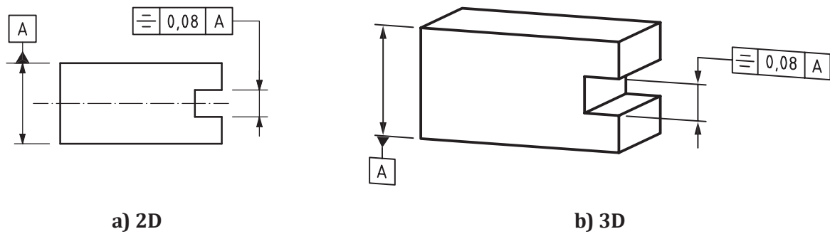
Figure 169 — Symmetry indication
