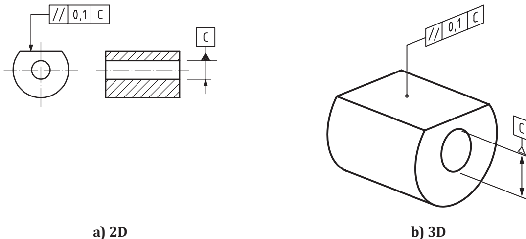
Figure 124 — Parallelism indication
