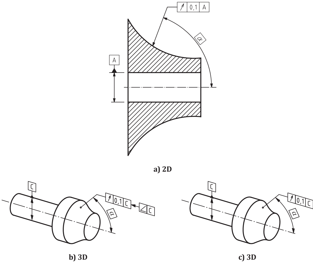
Figure 85 — Drawing indication
