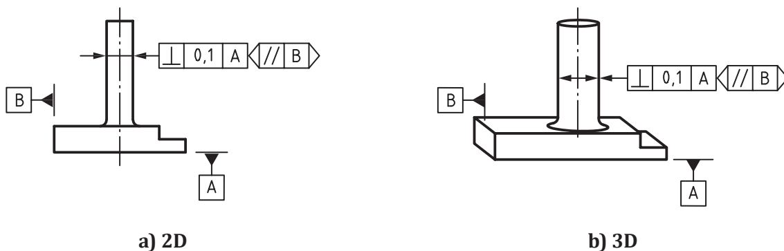
Figure 130 — Perpendicularity indication
