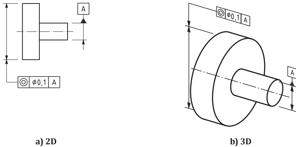
Figure 166 — Coaxiality indication
