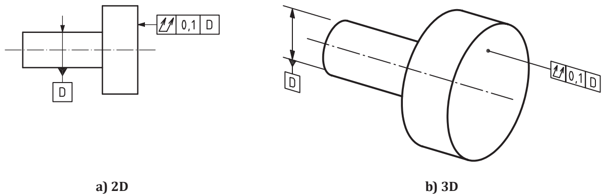
Figure 186 — Total run-out indication
