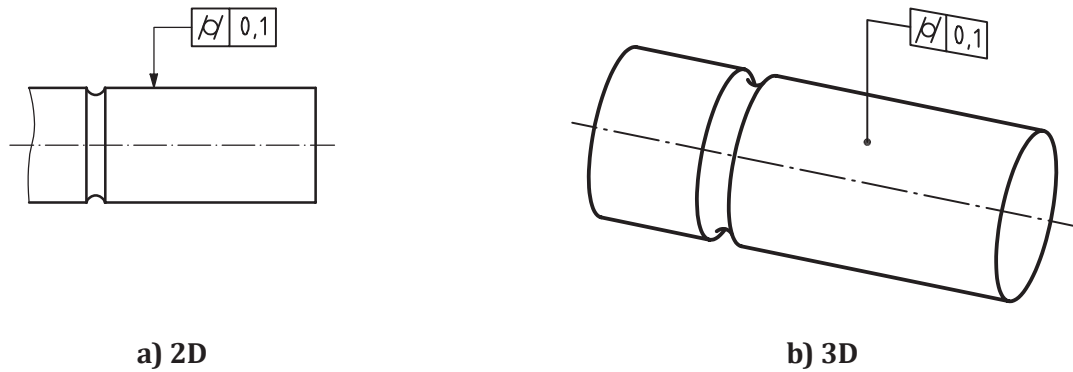
Figure 102 — Cylindricity indication
