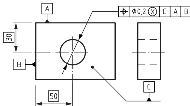
Figure 33 — Maximum inscribed associated toleranced feature — Drawing indication
