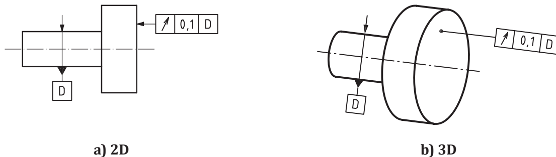
Figure 177 — Circular run-out indication
