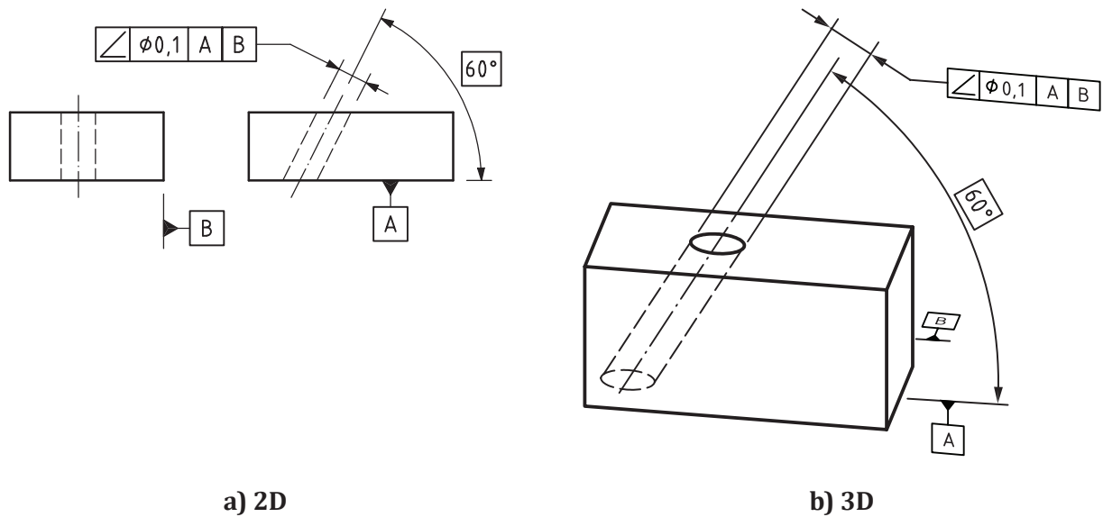
Figure 144 — Angularity indication
