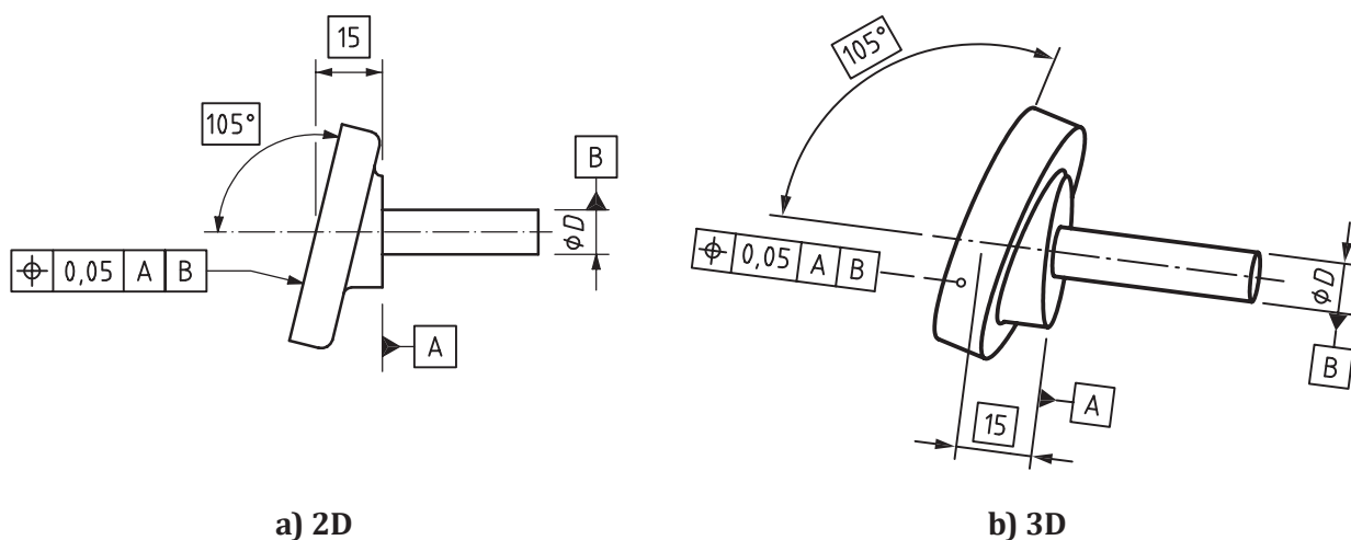
Figure 161 — Position indication
