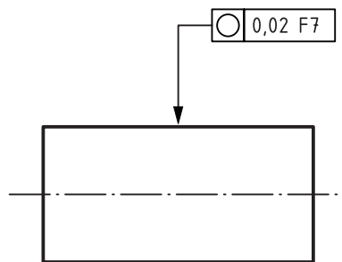
Figure E.17 — Example of a roundness specification that applied to a single or a range of harmonics
