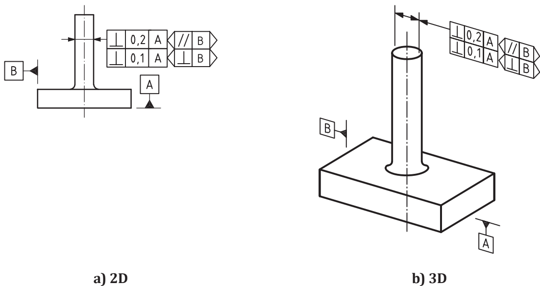
Figure 132 — Perpendicularity indication
