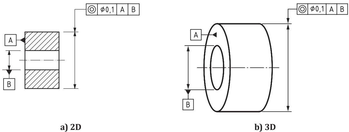
Figure 167 — Coaxiality indication
