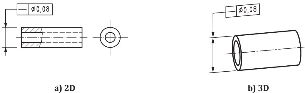
Figure 94 — Straightness indication
