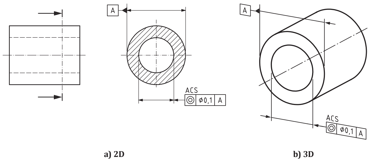
Figure 163 — Concentricity indication
