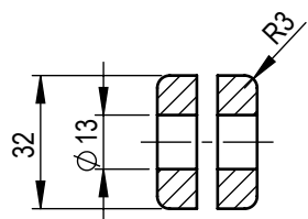
SECTION C-C SCALE 1 : 2
