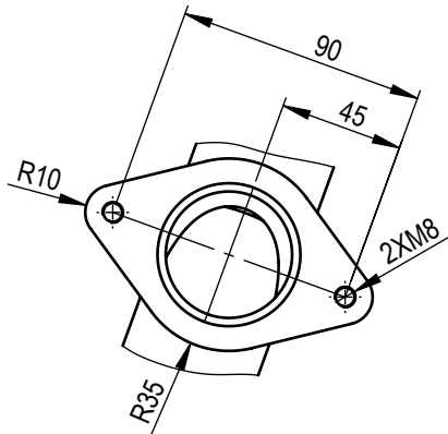
VIEW A
